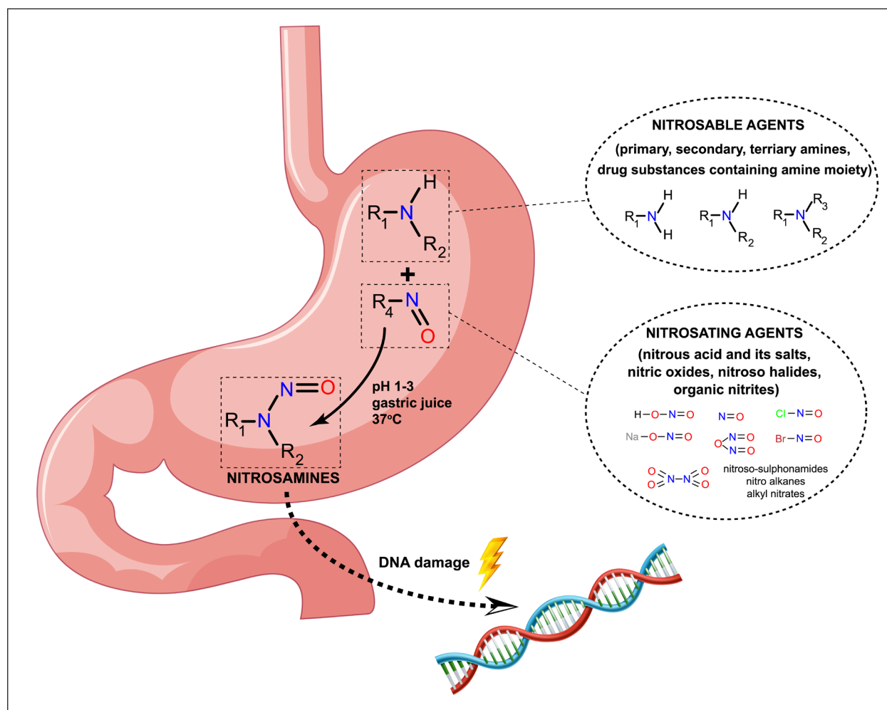
Figure 3. The mechanism of an endogenous drug nitrosation
