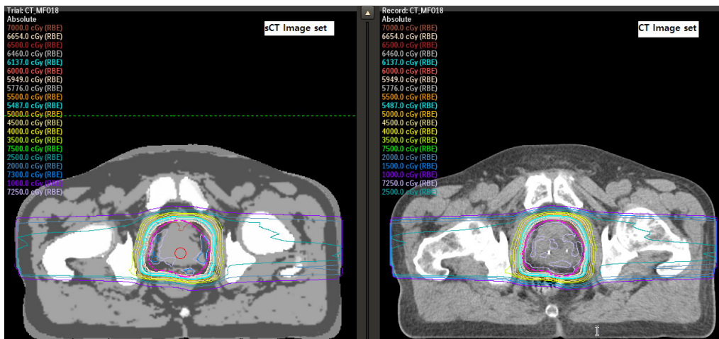
Figure 3. 2D Isodose lines display of MFO plan on CT plan and re-computed plan on sCT data set for a randomly chosen patient
