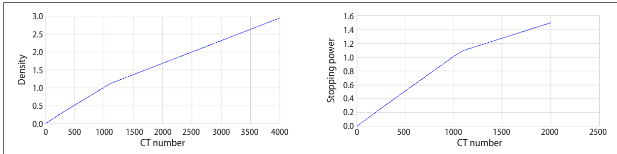
Figure 1. CT to density table and CT to stopping power table used for synthetic CT dose computation
