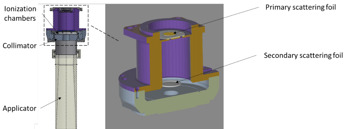
Figure 2. Scheme of an applicator with a diameter of 100 mm designed to be made of a biocompatible transparent material (MED610) for AQUIRE IOERT accelerator. Enlarged view of the layout of scattering foils in the collimator
