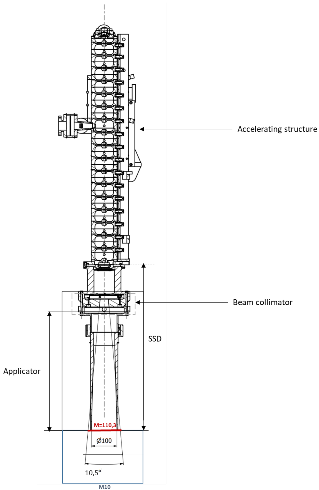
Figure 5. The beam limiting system geometry for the AQUIRE accelerator with M and M10 area
