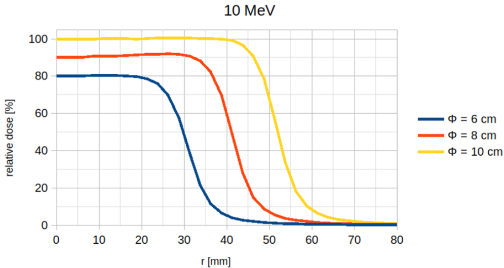
Figure 7. Monte Carlo simulations of electron beam off-axis profiles
