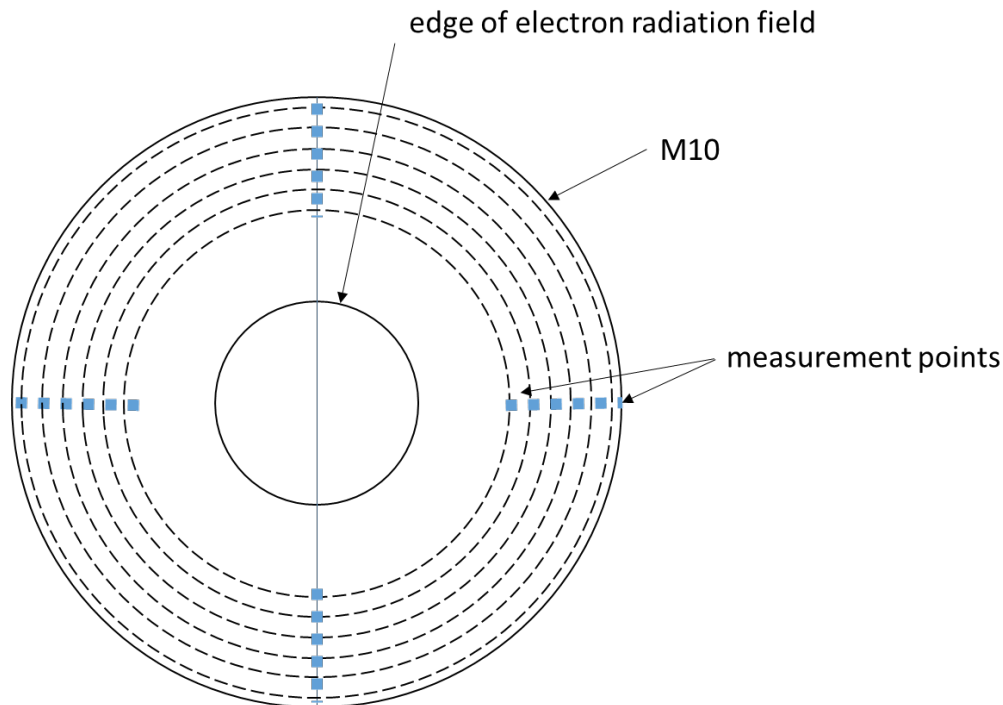
Figure 6. The geometry of the average absorbed dose outside the M10 area measurement
