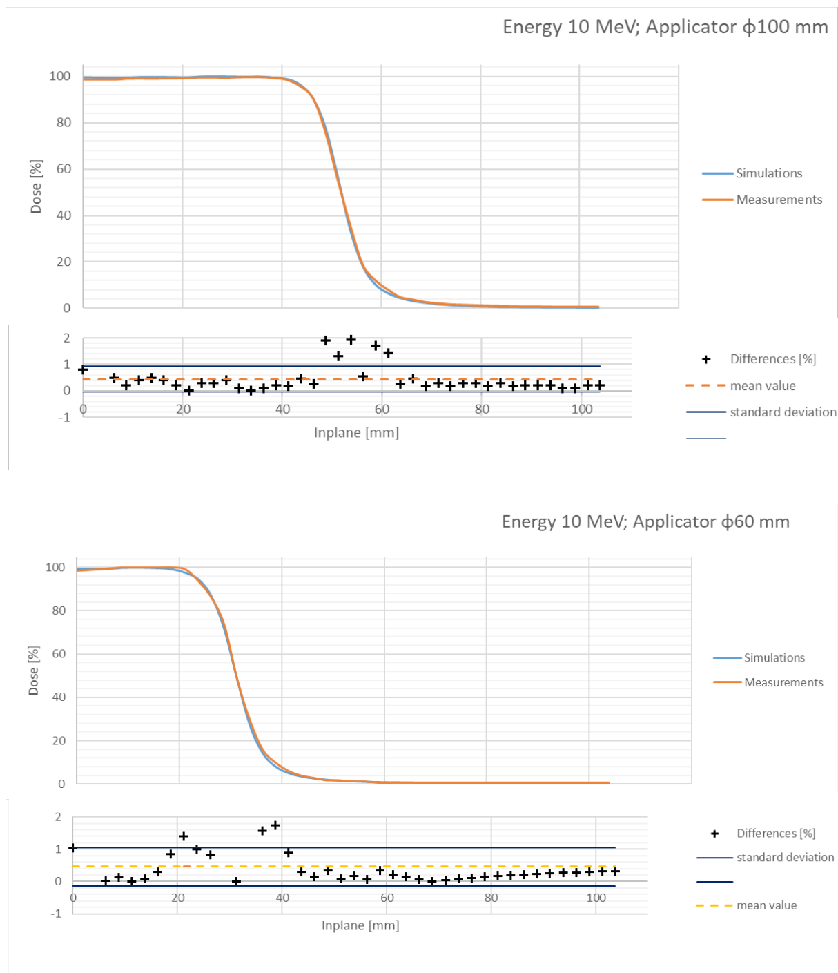
Figure 8. Inplane profile comparison for 10 and 6 cm circular field applicator; blue — simulations, orange — measurements.
