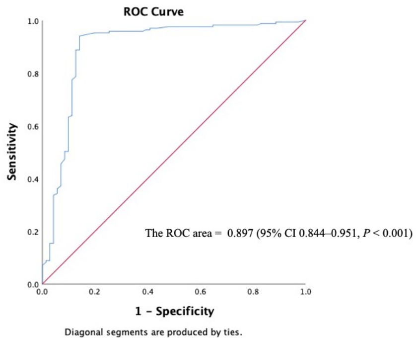
Figure S1. ROC curve of atrial contractile strain as a predictor of notch formation in the TAPSE curve
