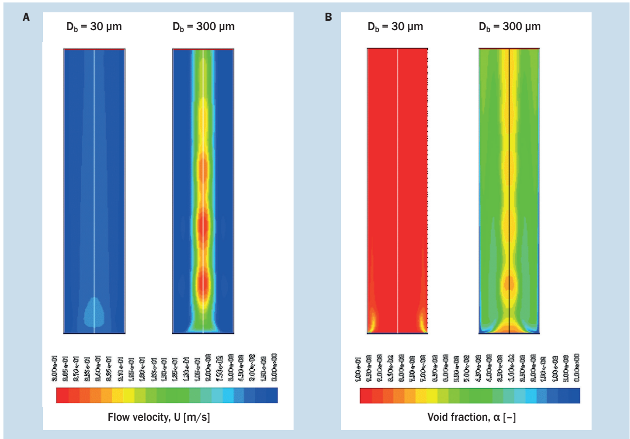
Figure 3. Effect of bubble size, D_b , on the flow velocity, U , (A) and void fraction, \alpha , (B) contour plots for pulsatile (sinusoidal) flow with input data: \alpha = 0.10 , U_{l,\text{mean}} = 3 \text{ cm/s} , pulsation frequency: 1 Hz, pulsation amplitude: \pm 50\% . The height dimension has been compressed by a factor of 10
