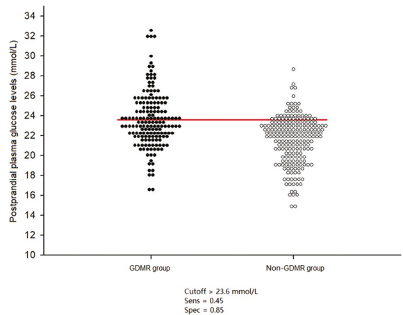
Figure 3. Dot histogram showing the area under the receiver operating characteristic curve (AUC), sensitivity, and specificity of FPG-1 + OGTT 1h and 2h-1
