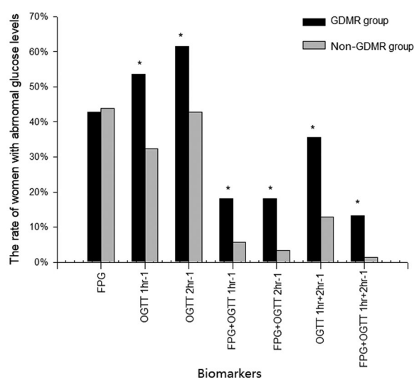
Figure 1. Comparison of the number of biomarker abnormalities (%) of women in the gestational diabetes mellitus recurrence (GDMR) and non-GDMR groups; * p < 0.05 , GDMR group compared to the non-GDMR group
