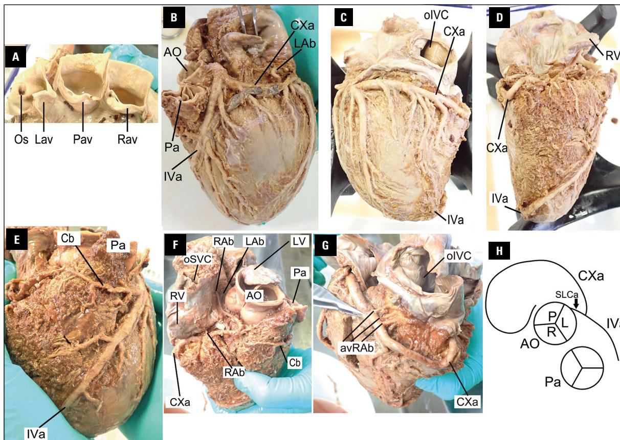
Figure 1. Single left coronary artery (SLCa) and blood vessels branching from SLCa, observed from various directions. Each panel ([A] to [G]) in the figure demonstrates each aspect. Schematic diagram representing the L1 type Lipton classification of a single coronary artery (H). The orifice is located in the left sinus (of). Some right atrial branches (RAB) are atrioventricular branches (avRAB). AO — abdominal aorta; avRAB — atrioventricular branch; Cb — conus branch; CXa — circum-flex artery; IVa — anterior interventricular branch; L — left Valsalva sinus; LAb — left atrial branch; Lav — left aortic valve; LV — right ventricle; oIVC — opening of the inferior vena cava; Os — orifice of single left coronary artery; oSVC — opening of the superior vena cava; P — posterior aortic sinus; Pa — pulmonary artery; Pav — posterior aortic valve; R — right Valsalva sinus; Rav — right aortic valve.
