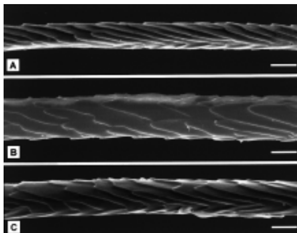
Figure 5. Variability of cuticular scale double chevron patterns in the mid-portion of the shafts of dorsal wool hairs in different breeds. Scale bars = 10 \mu\text{m} .
