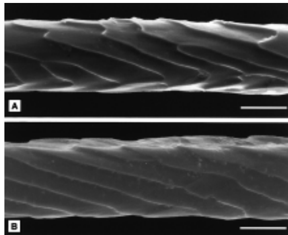
Figure 9. Different SEM images of double chevron scale pattern of wool hairs. Scale bars = 10 \mu\text{m} . A) View of the crests and bottoms of the troughs formed by the scale margins when observed perpendicularly. (Angora rabbit). B) Torsion image obtained when the scale margins are observed under an oblique angle (New Zealand White rabbit).
