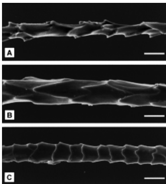
Figure 6. Variability of cuticular scale petal patterns at the base of wool hairs in different breeds. Scale bars = 10 \mu\text{m} .
