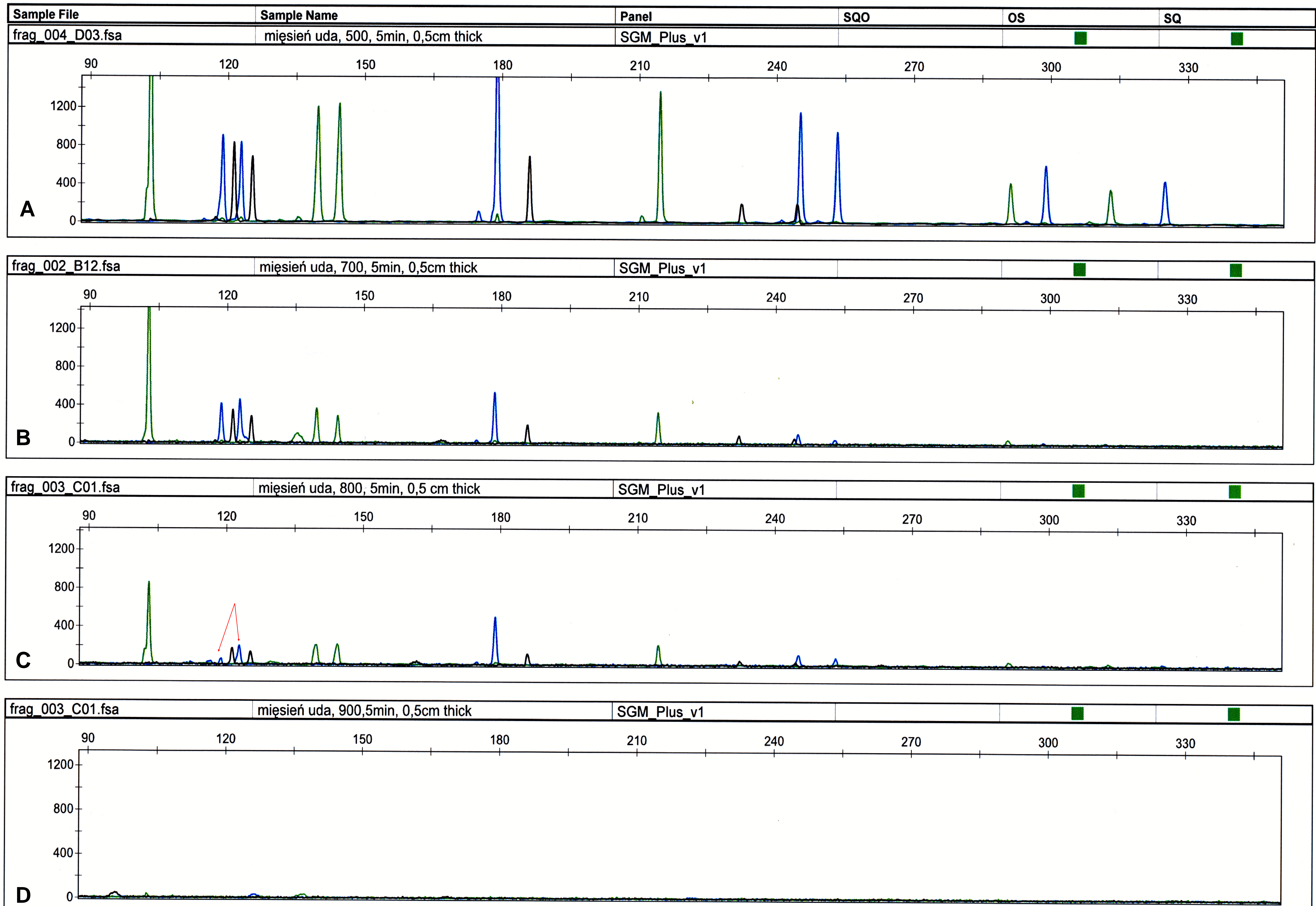
Figure 8. The SGMPlus profiles obtained for the 0.5 cm-thick thigh muscle exposed to 500°C (A), 700°C (B), 800°C (C) and 900°C (D) for 5 min. The arrows indicate the heterozygotes with peaks ratio lower than 60%
