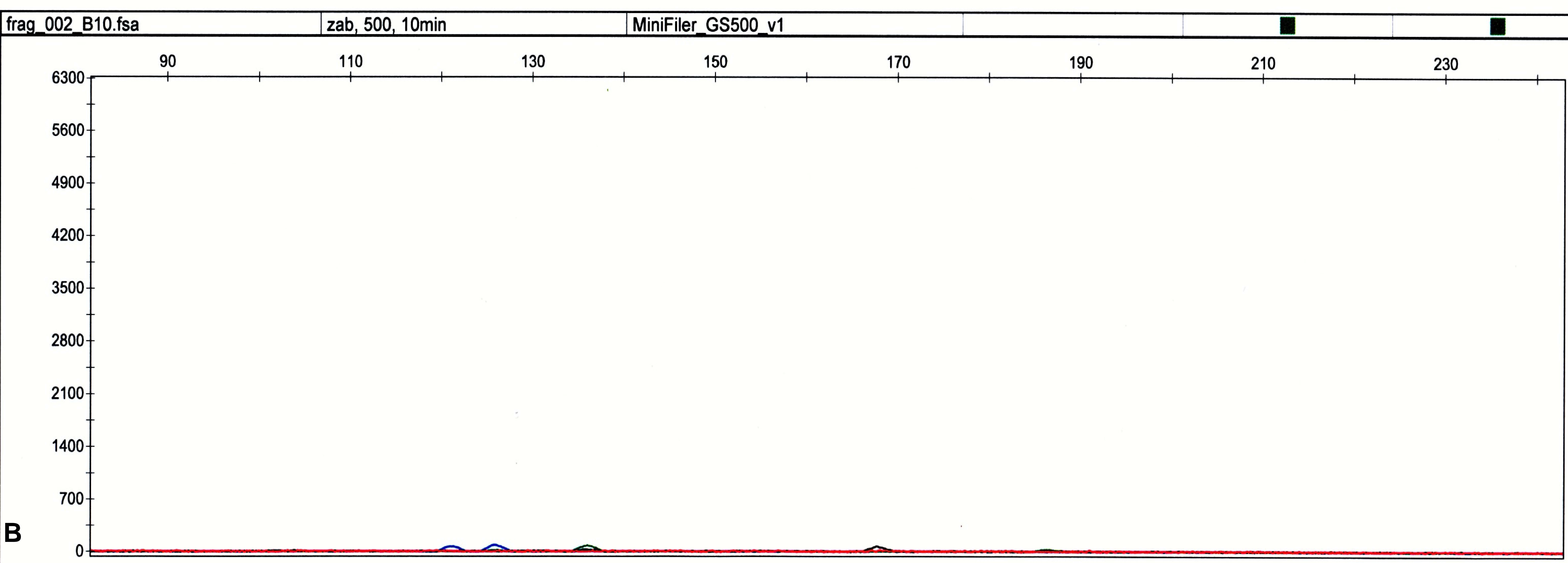
Figure 3. MiniFiler profiles obtained for the teeth exposed to 300°C (A) and 500°C (B) for 10 min
