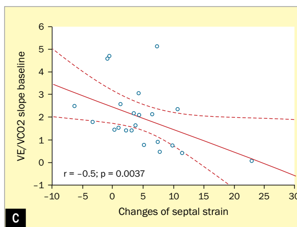
Figure 2. Correlations between changes of septal longitudinal peak strain (LPS) values in the nonresponders and the responders (six months follow-up measurement minus basic measurement) and: the baseline peak oxygen uptake, the baseline peak carbon dioxide exertion, the baseline slope of VE/VCO2 relationship from the initiation to peak exercise
