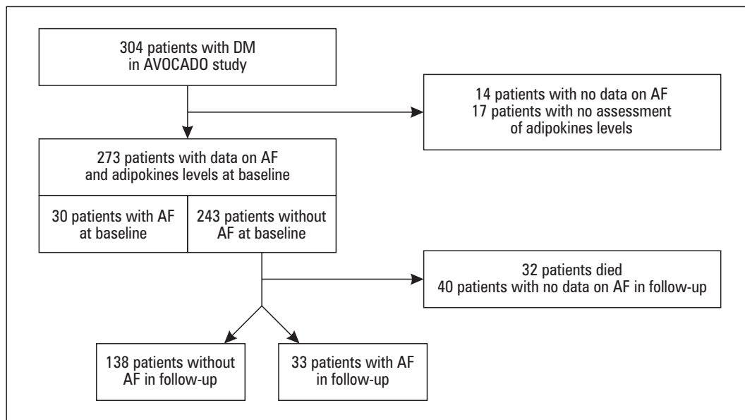
Figure 1. Flowchart of subgroups selection. AF — atrial fibrillation; DM — diabetes mellitus; pts — patients
