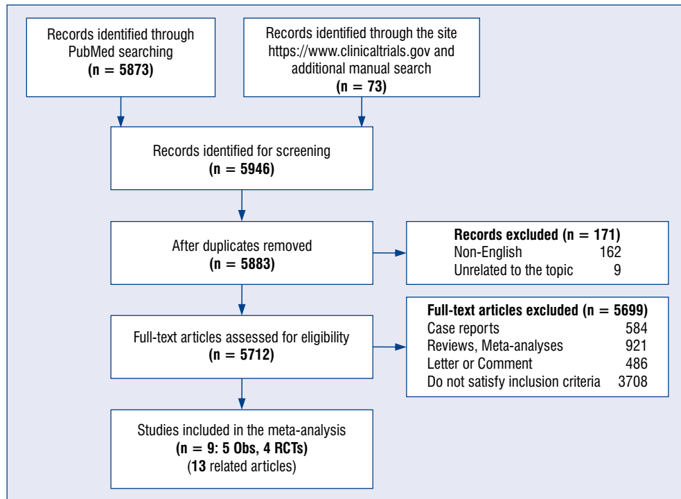
Figure 1. Flow-chart of the study selection process; Obs — observational studies; RCTs — randomized controlled trials.
