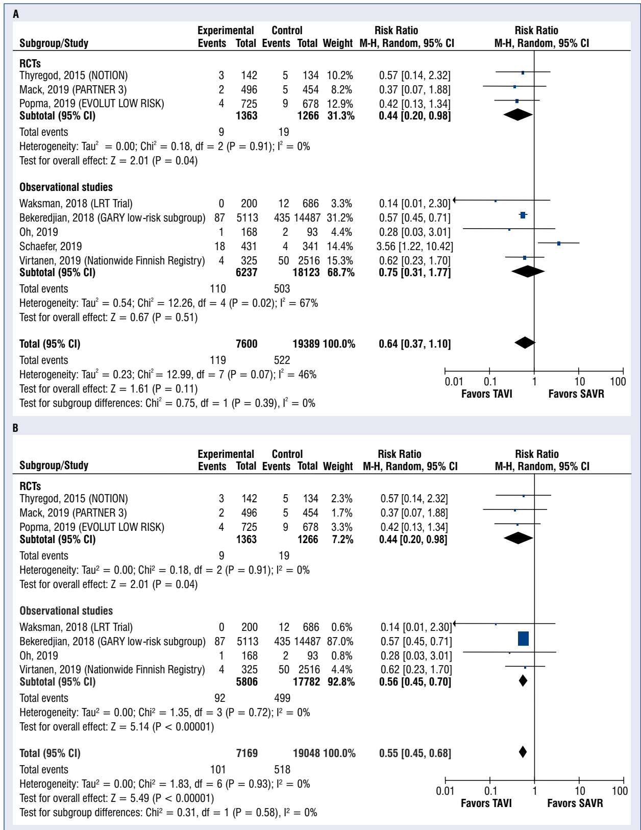
Figure 2. Forest plot of the primary end point: risk ratio of 30-day all-cause mortality between transcatheter aortic valve implantation (TAVI) and surgical aortic valve replacement (SAVR) in all studies (A) and after sensitivity analysis (B); CI — confidence interval; M-H — Mantel-Haenszel; RCTs — randomized controlled trials.
