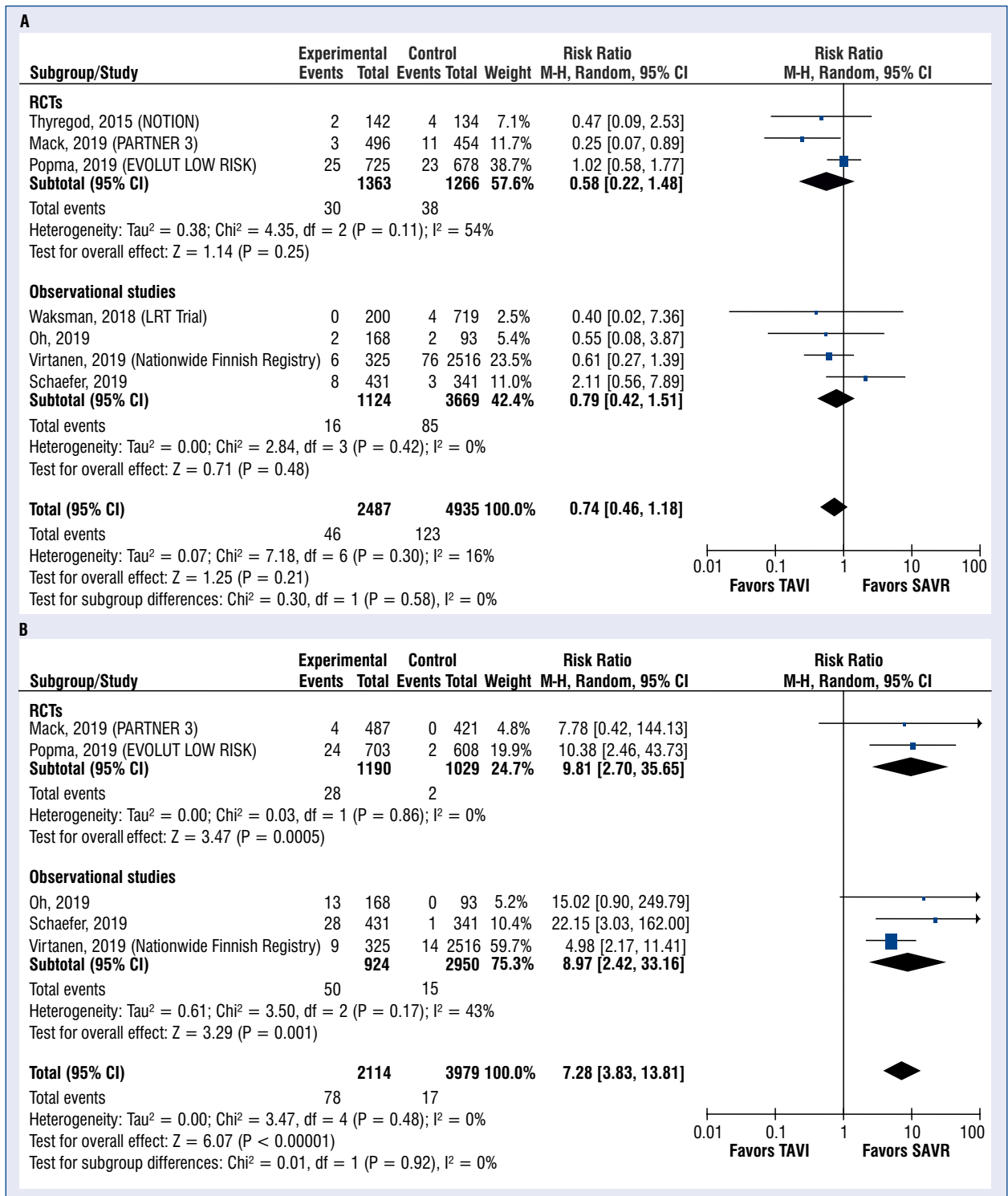
Figure 5. Forest plots of the 30-day safety endpoints: risk ratio of stroke (A) and paravalvular leak (B) between transcatheter aortic valve implantation (TAVI) and surgical aortic valve replacement (SAVR); CI — confidence interval; M-H — Martel-Heansel; RCTs — randomized controlled trials.
