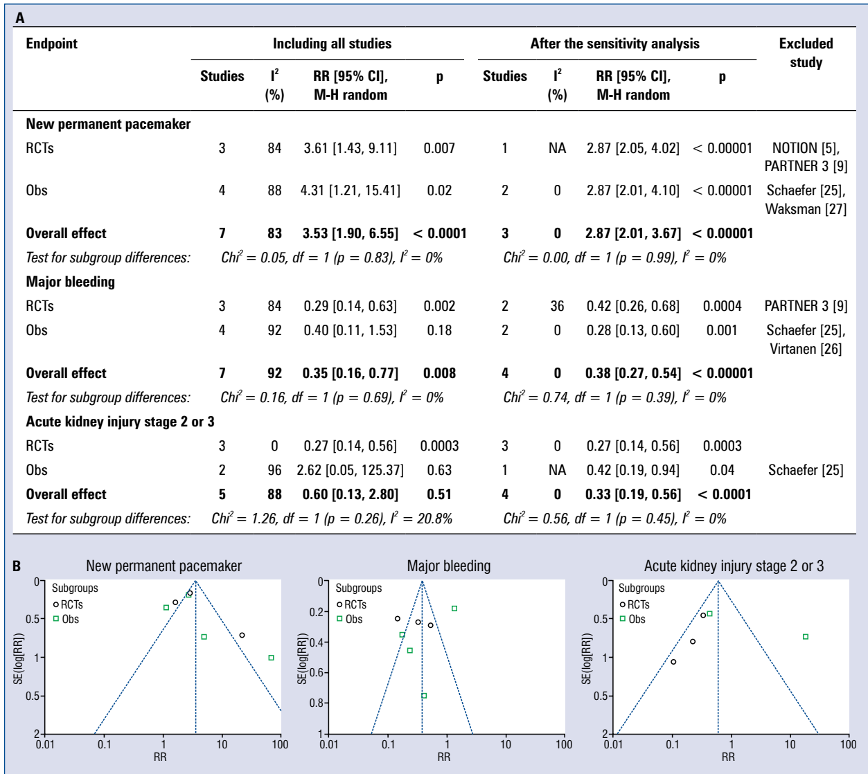
Figure 4. Thirty day safety endpoints: new permanent pacemaker implantation, major bleeding and acute kidney injury stage 2 or 3; A. Results of the comparisons between transcatheter aortic valve implantation and surgical aortic valve replacement before and after the sensitivity analysis; B. Funnel plots on the log of risk ratio (RR) of each safety end-point, plotted against the standard error (SE) of the log RR; dotted lines represent the risk estimate and its 95% confidence limits; CI — confidence interval; M-H — Mantel-Haenszel; NA — not applicable; Obs — observational studies; RCTs — randomized controlled trials.
