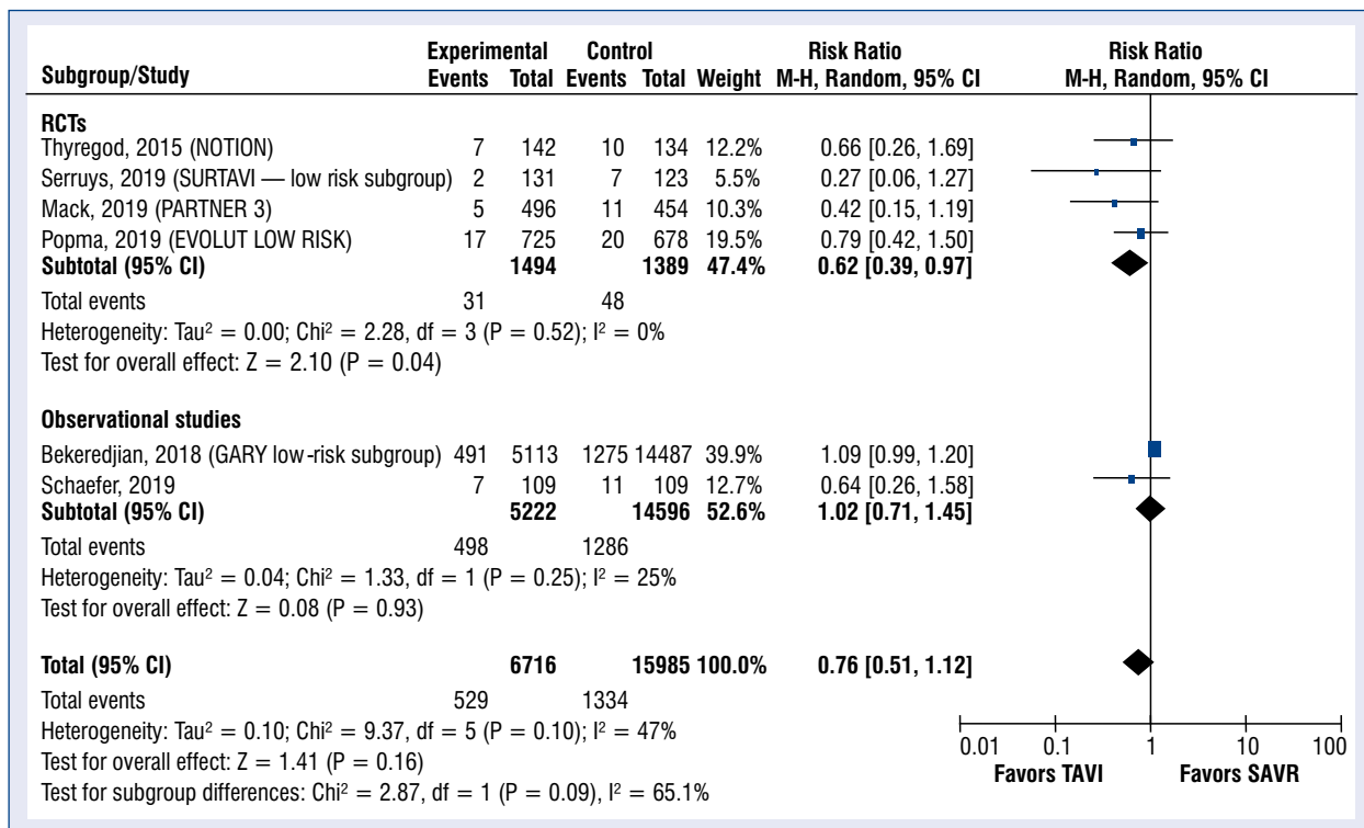
Figure 3. Forest plot of the primary end point: risk ratio of 1-year all-cause mortality between transcatheter aortic valve implantation (TAVI) and surgical aortic valve replacement (SAVR); CI — confidence interval; M-H — Mantel-Haenszel; RCTs — randomized controlled trials.
