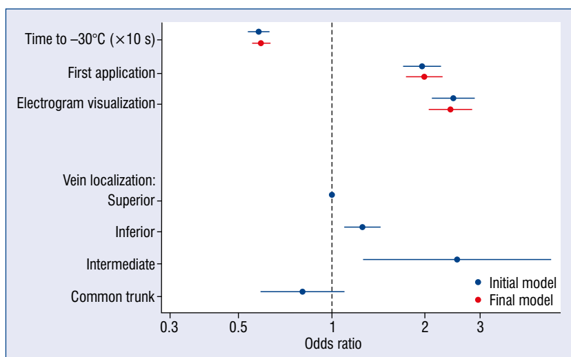
Figure 2. Multivariate logistic regression models predicting successful cryoballoon application.
