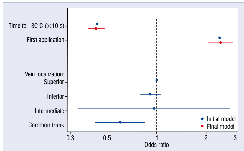
Figure 3. Multivariate logistic regression models predicting a successful cryoballoon application achieving vein isolation within 60 s.
