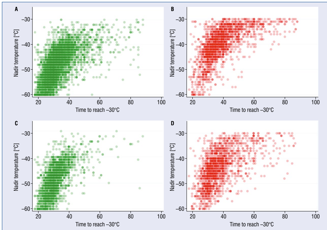
Figure 5. Scatter plot of recorded nadir temperature and time to -30°C; A, B. Green dots represent successful applications, and red dots represent failure to isolate; C, D. Green dots represent isolation under 60 s, and red dots depict failure to isolate under 60 s with electrogram monitoring.
