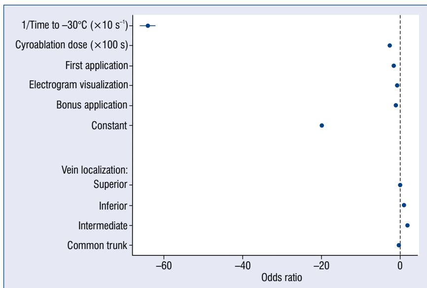
Figure 6. Multivariable linear regression model for nadir temperature.
