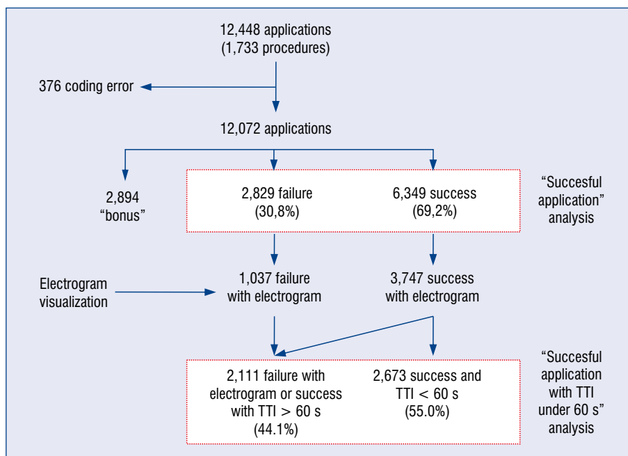
Figure 1. Flowchart and classification of cryoballoon applications. Successful application refers to achieving vein isolation; TTI — time to isolation.
